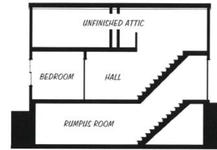
ORIGINAL BUILDING SECTION
